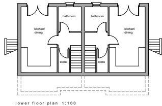
lower floor plan 1:100
